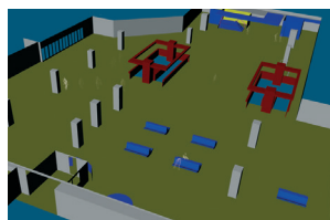
TIMMS – 3D LiDAR Based Model of Philadelphia Subway Concourse
