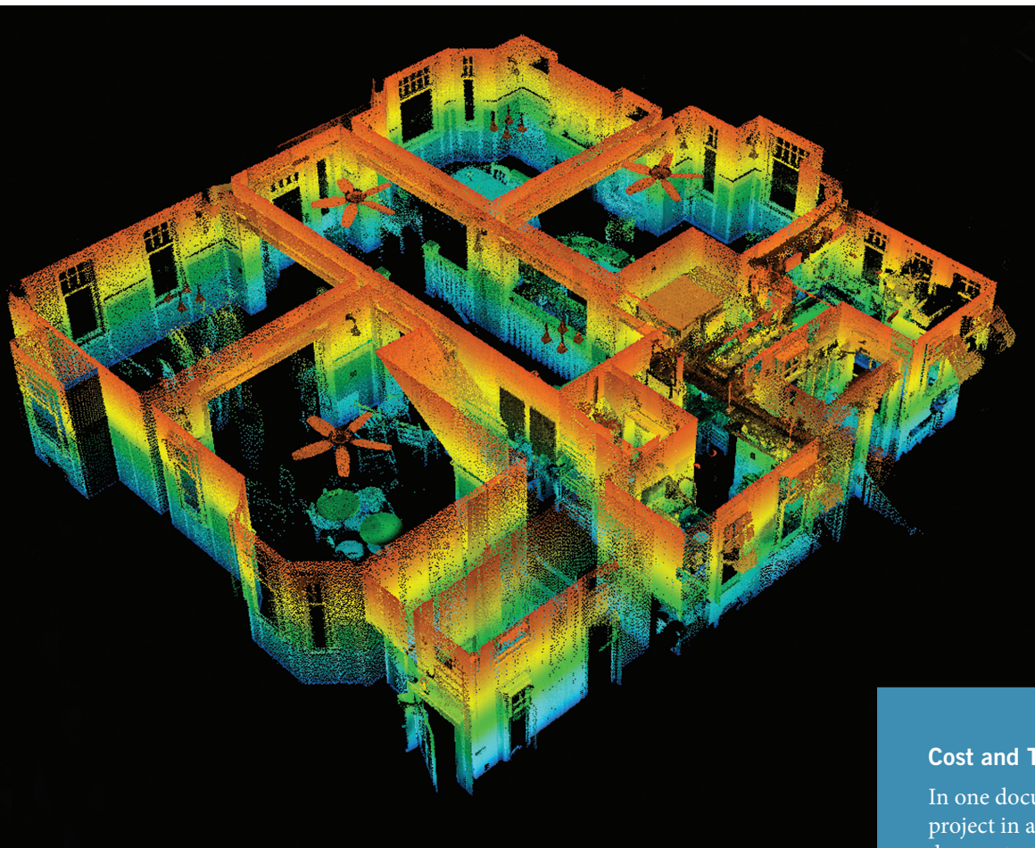
TIMMS scan and resulting maps/models
